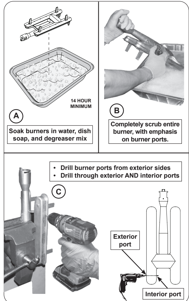
Fig. 4-3 Cast stainless steel burner cleaning
