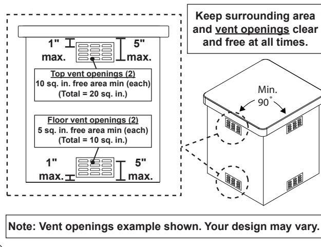
Fig. 12-1 Ventilation Detail
