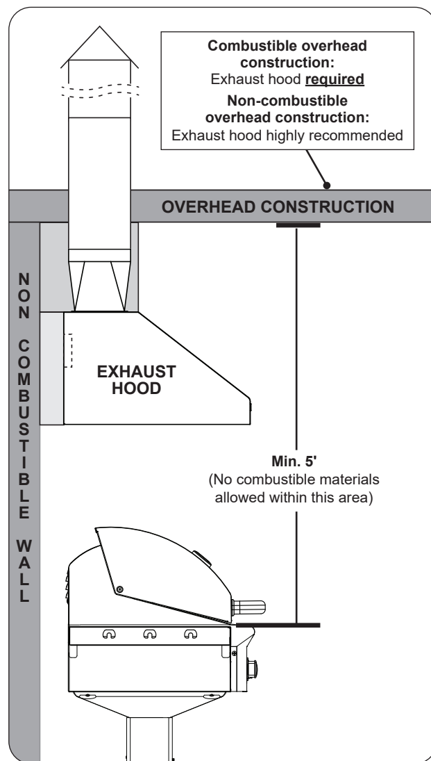
Fig. 13-1 Overhead requirements
