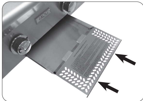
Fig. 19-4 Install drip tray
