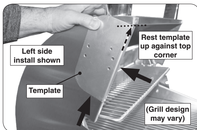
Fig. 1-1 Place drilling template (on hood)
