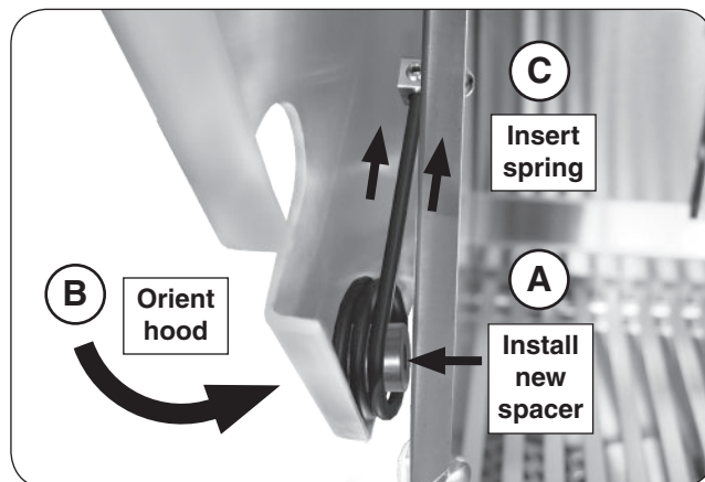
Fig. 3-3 Install hood
