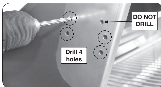
Fig. 1-2 Drill holes (on hood)
