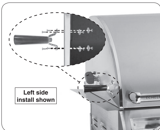
Fig. 1-3 Install bracket to hood
