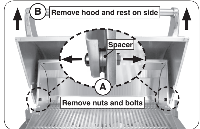
Fig. 2-2 Remove hood
