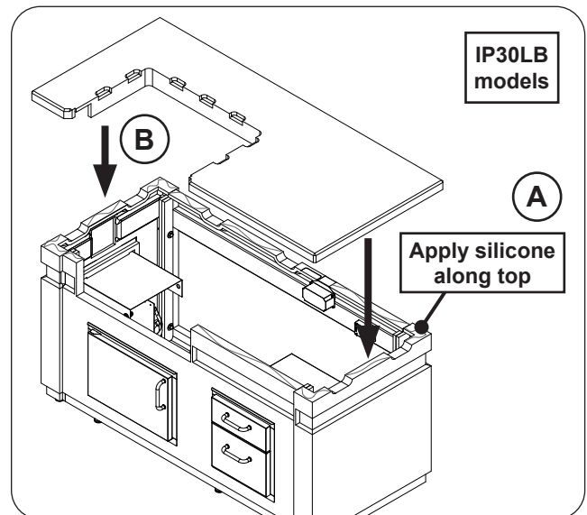
Fig. 10-2 Place countertop
