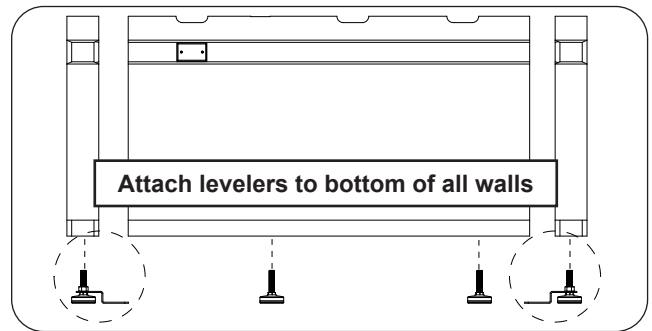
Fig. 7-1 Attach levelers
