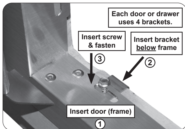
Fig. 9-2 Door / drawer install detail
