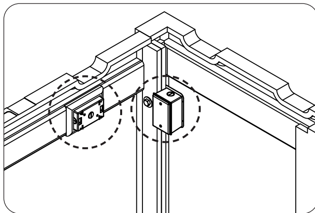
Fig. 8-3 Install electrical (as needed)
