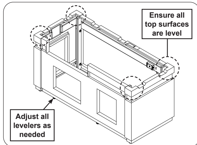
Fig. 8-1 Level assembly
